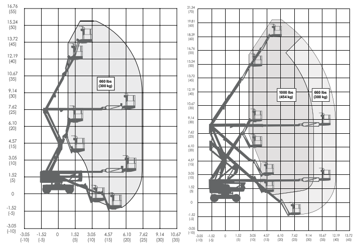
SJ45 AJE+ WORKING ENVELOPE
