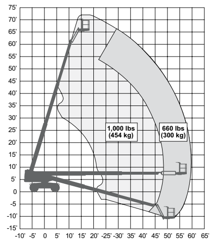
SJ66 T+ WORKING ENVELOPE
