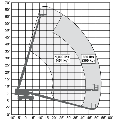
SJ61 T+ WORKING ENVELOPE
